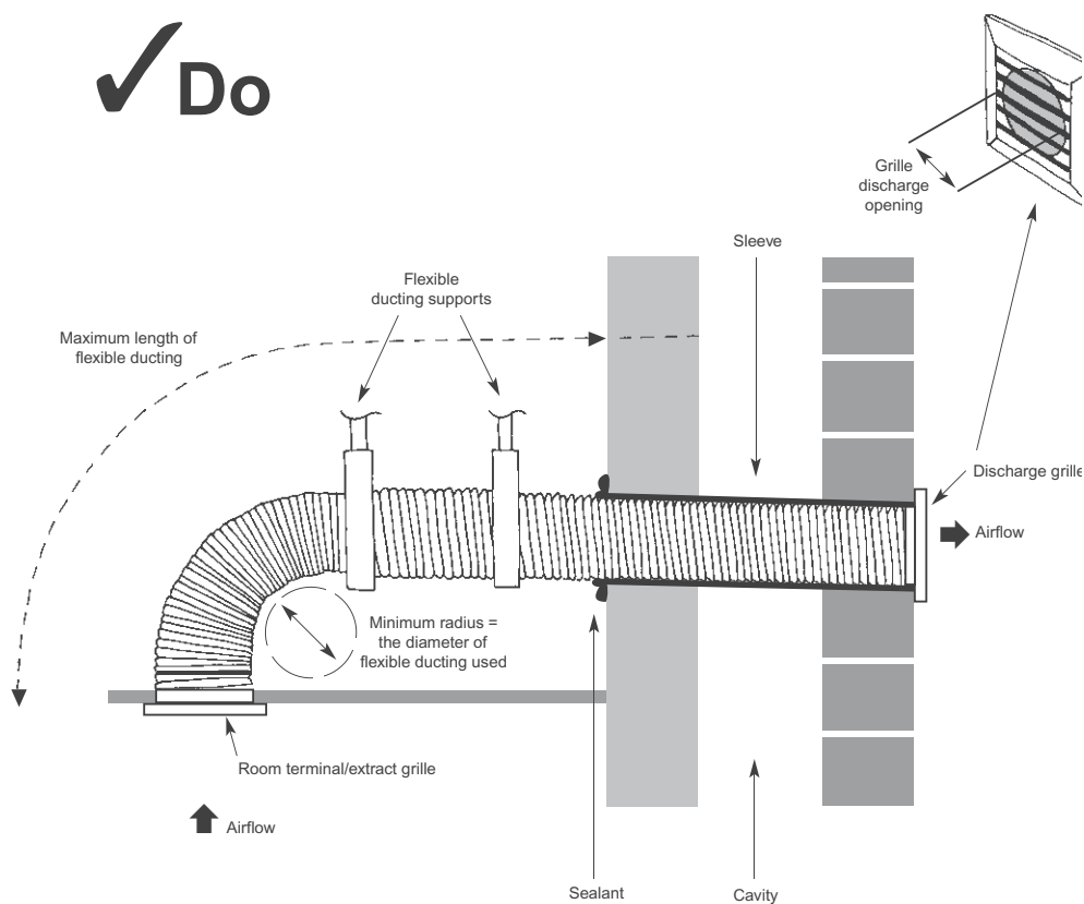
Diagram 1: Duct installations
